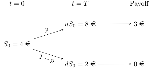
Figure 2: Binomial tree of stock prices with S_0 = 4 \text{ €} , u = 2 , d = \frac{1}{2} , and K = 5 \text{ €} .
