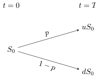
Figure 1: Binomial tree of stock prices with one period
