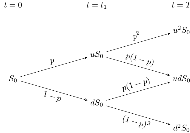
Figure 3: Binomial tree of stock prices with two periods
